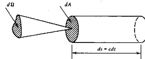
Figure 1.4 Electromagnetic energy in a cylinder.
