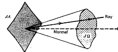
Figure 1.2 Geometry for normally incident rays.
