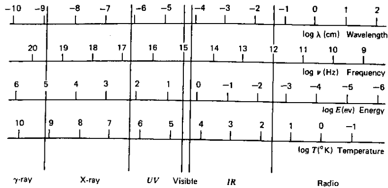
Figure 1.1 The electromagnetic spectrum.
