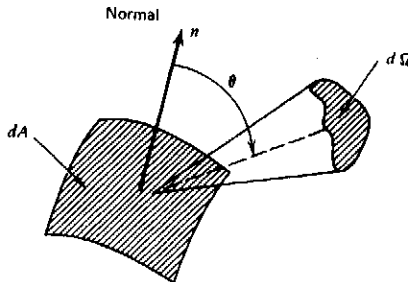
Figure 1.3 Geometry for obliquely incident rays.
