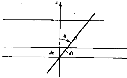
Figure 1.13 Geometry for plane-parallel media.
