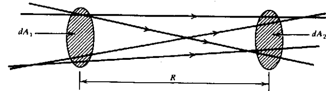
Figure 1.5 Constancy of intensity along rays.
