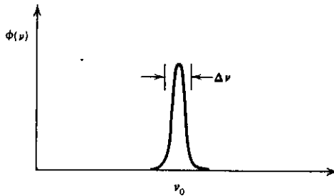
Figure 1.12b Line profile for 1.12a.
