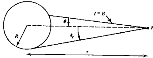
Figure 1.6 Flux from a uniformly bright sphere.
