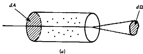
Figure 1.7a Ray passing through a medium of absorbers.
