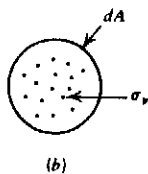
Figure 1.7b Cross sectional view of 7a.
