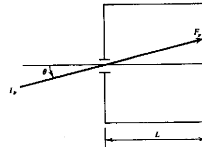
Figure 1.14 Geometry for a pinhole camera.
