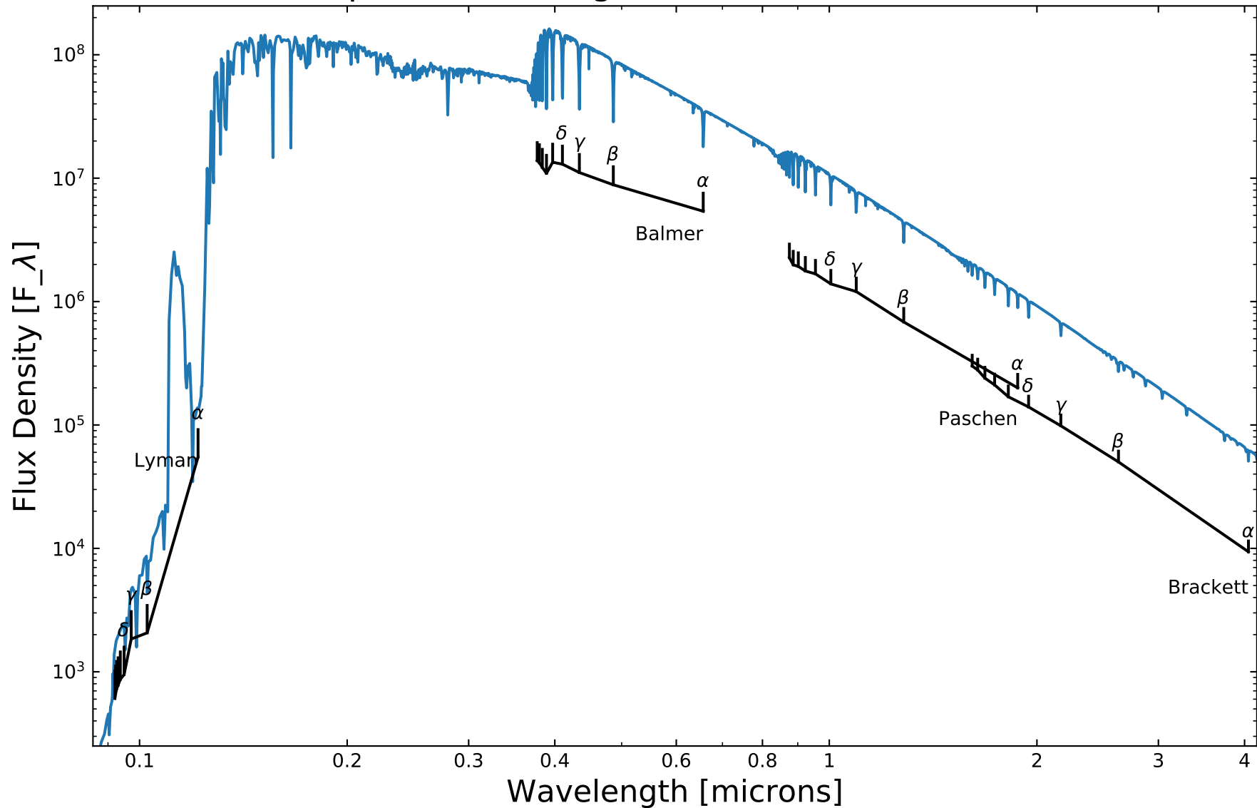
Spectrum of Vega-like star (T=10,000 K)
